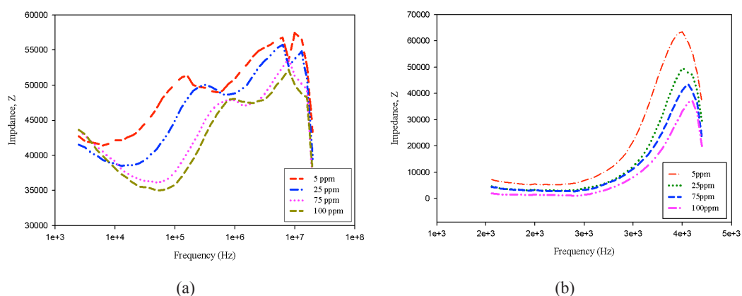
Figure 5. Impedance for different concentration level of nitrate (a) coated with Incralac; (b) coated with membrane
