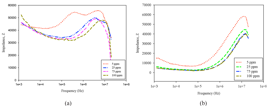
Figure 6. Impedance for different concentration level of phosphate (a) coated with Incralac; (b) coated with membrane
